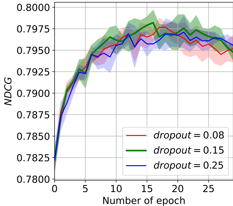
NDCG
